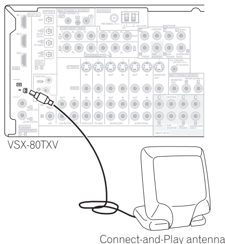
Connect-and-Play antenna
